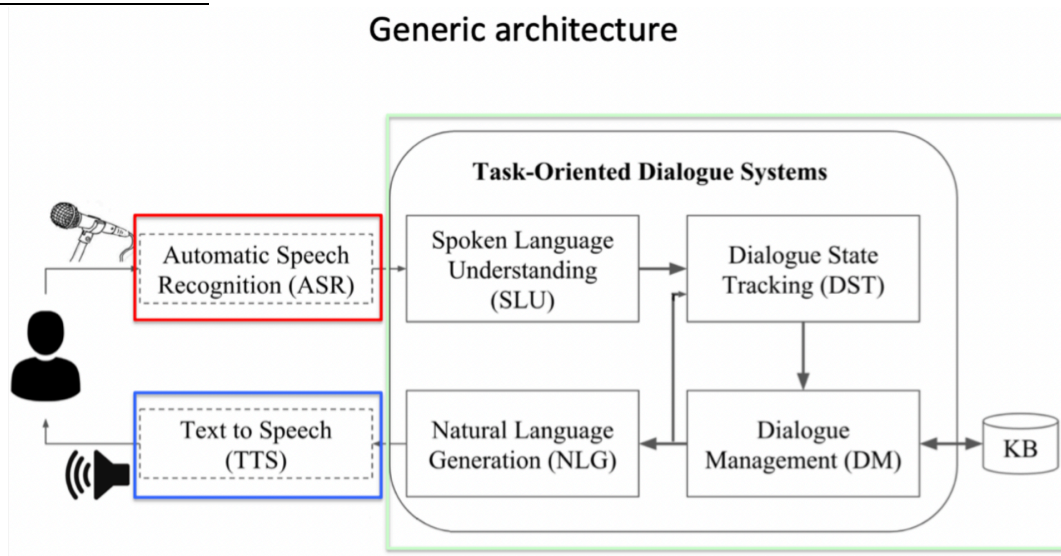
Generic dialog system architecture (Spoken Dialogue Systems set of slides of the NLP course)
