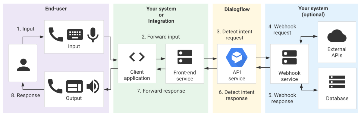
Figure 1 Interaction diagram ( https://cloud.google.com/dialogflow/cx/docs/basic/ )
