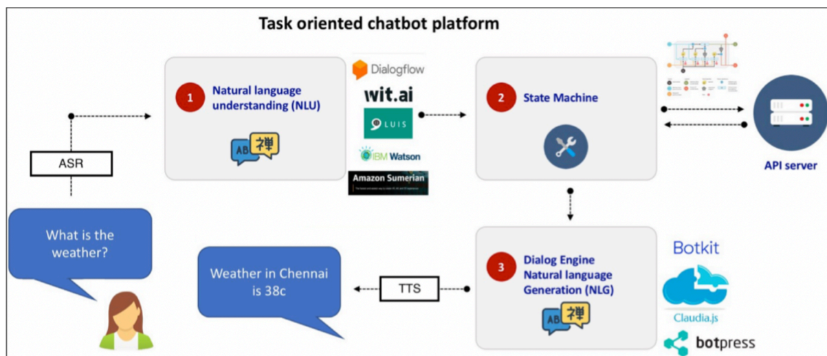
Task oriented chatbot system (SpokenDialogueSystems set of slides of the NLP course)
