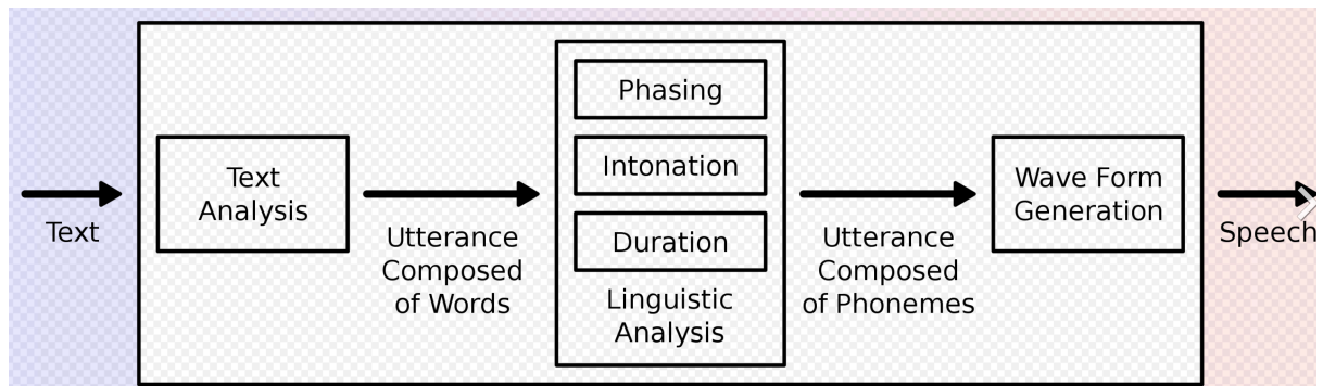
TTS model (Wikipedia)
